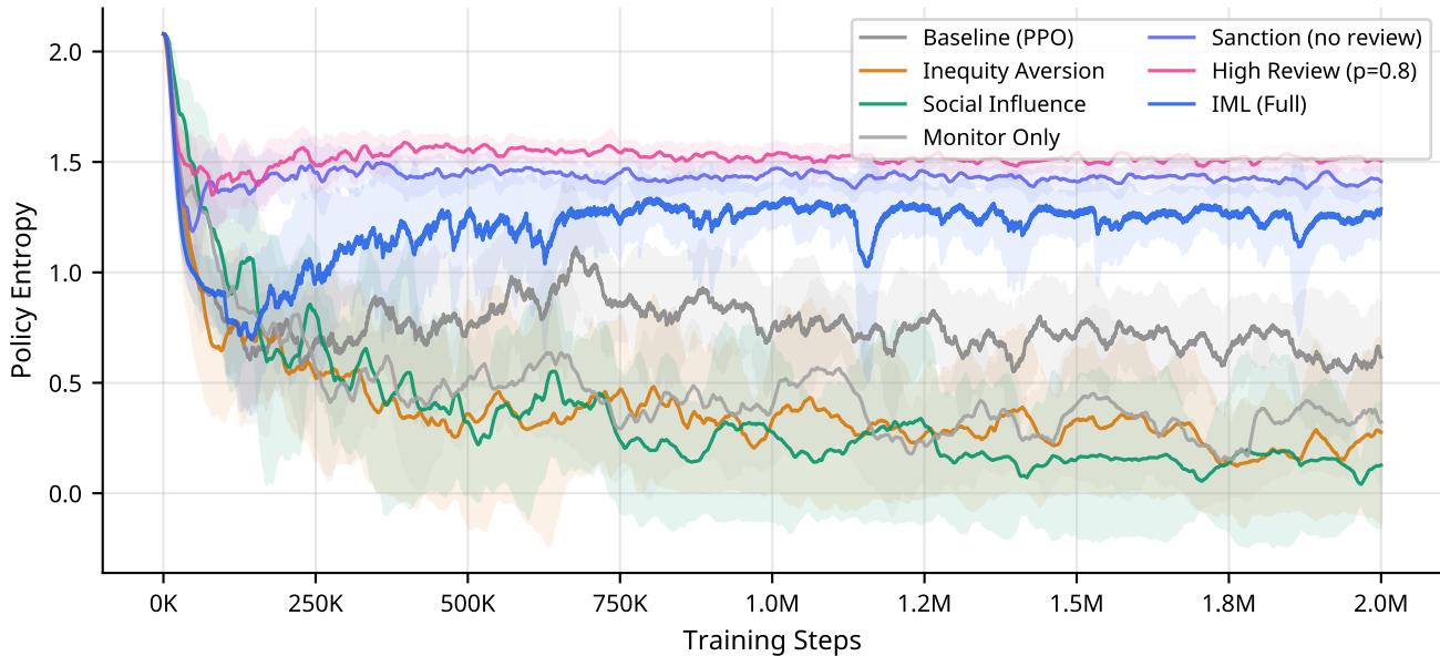
Harvest — Policy Entropy During Training
