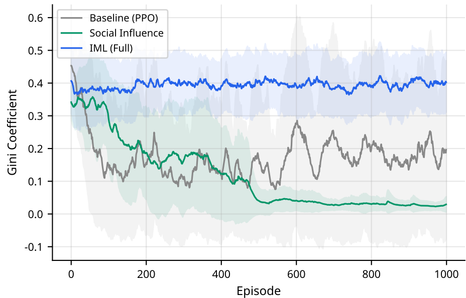
Cleanup — Reward Inequality (Gini)
