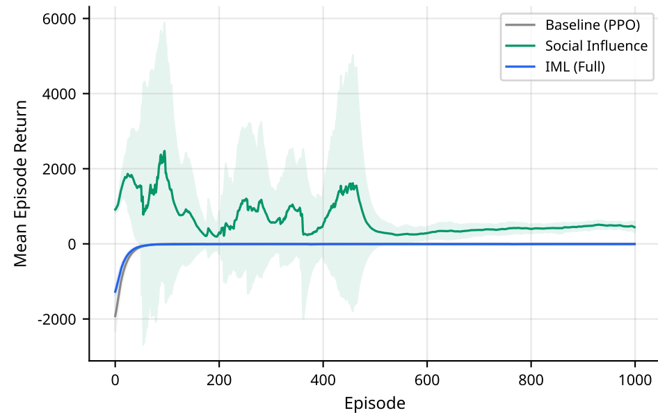
Cleanup — Episode Returns
