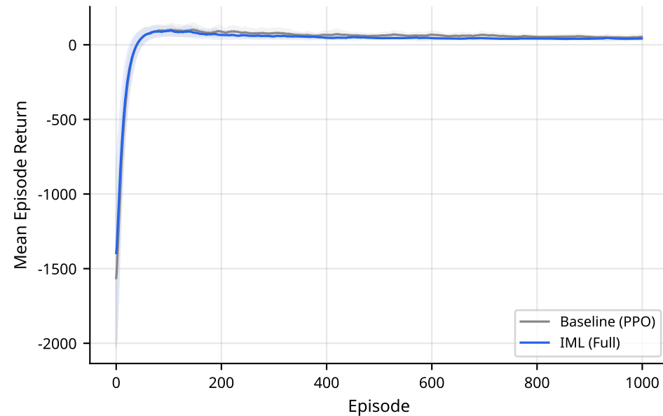
Harvest — Episode Returns
