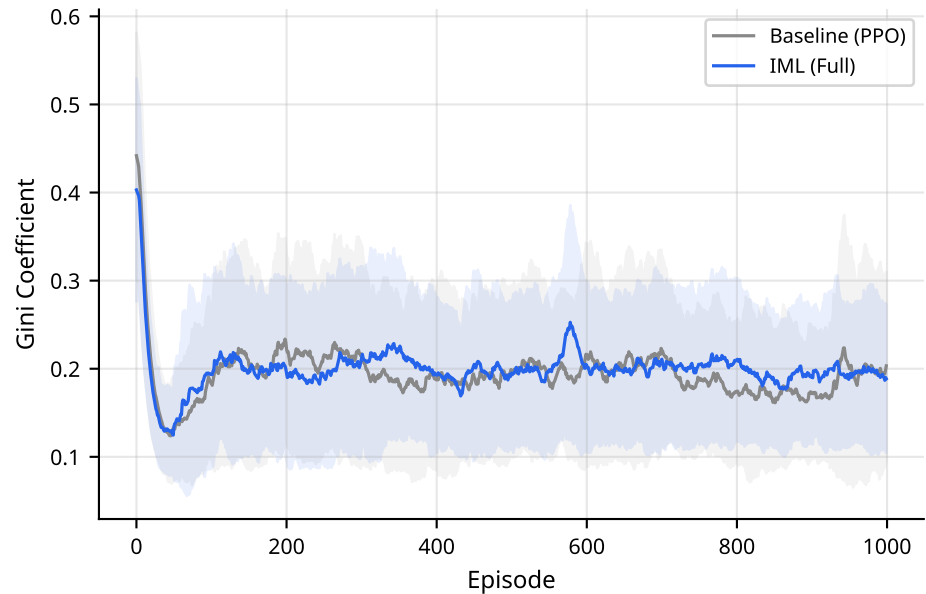
Harvest — Reward Inequality (Gini)
