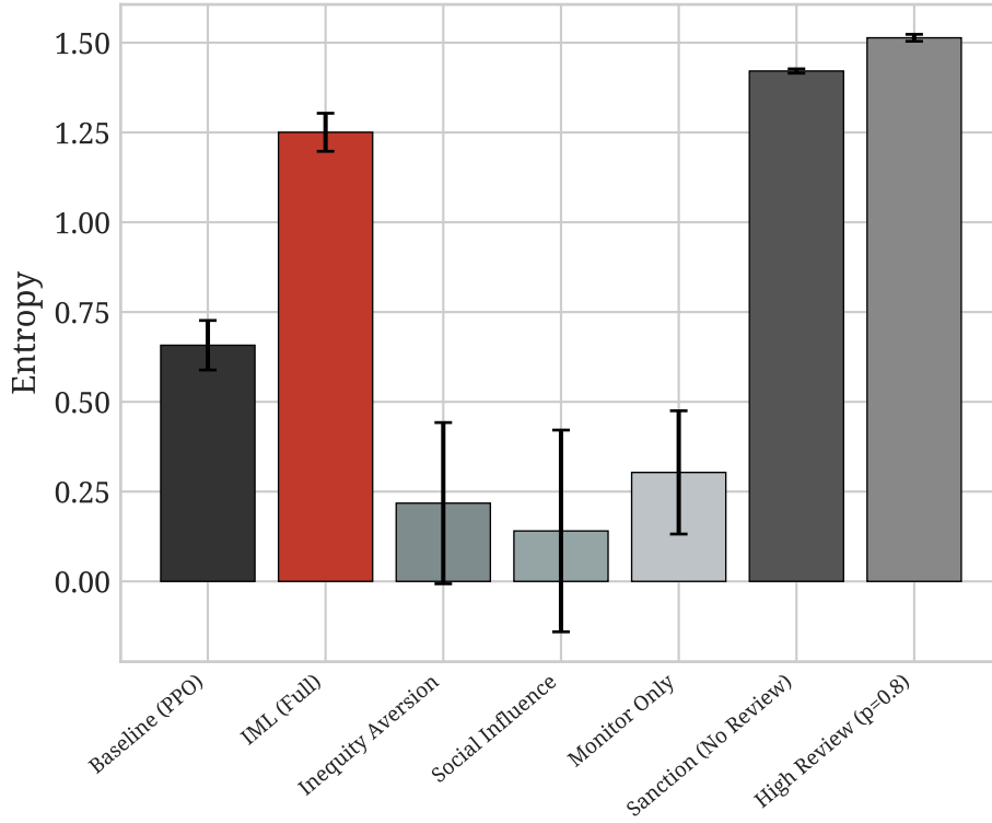
Harvest: Final Entropy
