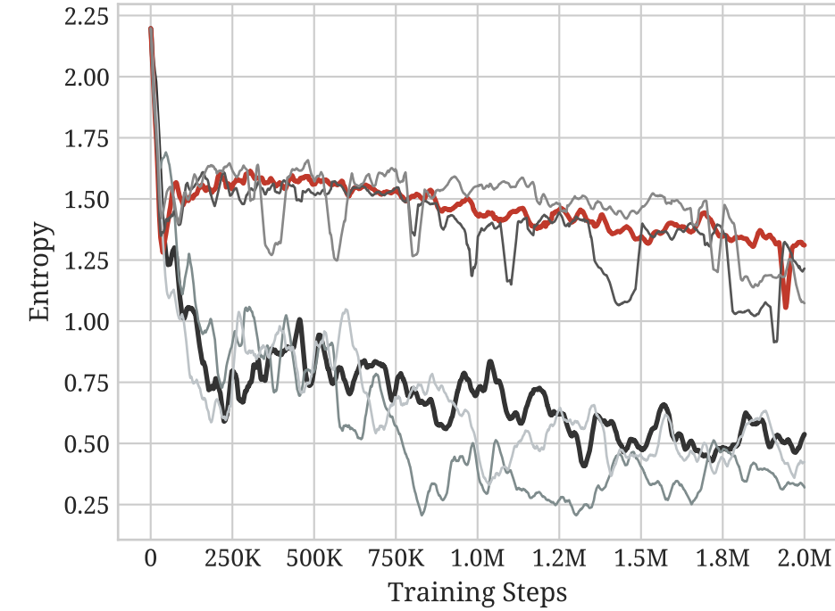
Cleanup: Entropy Over Training
