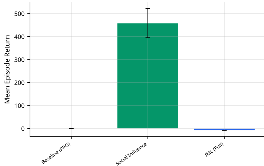
Cleanup — Converged Returns
