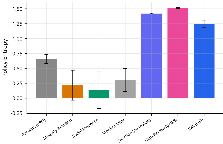
Harvest — Converged Entropy
