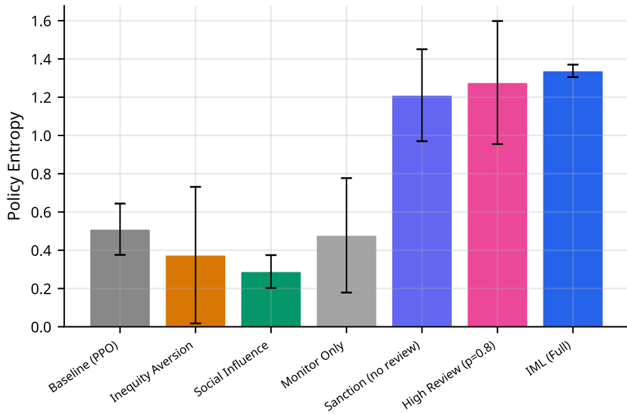
Harvest — Converged Entropy
