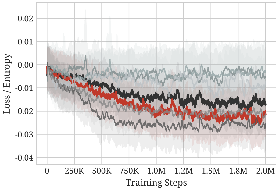
Policy Loss
