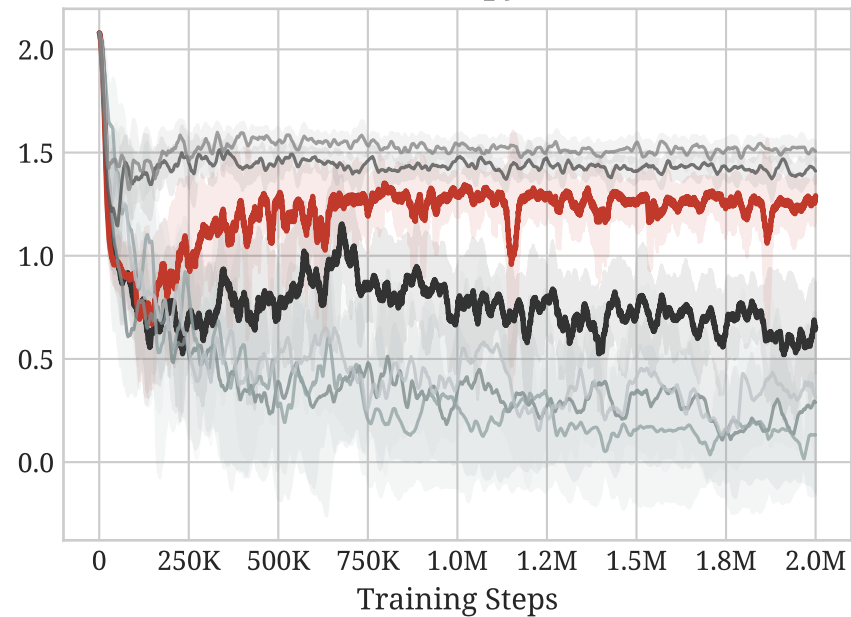
Entropy
