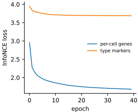
contrastive training (seed 0)
