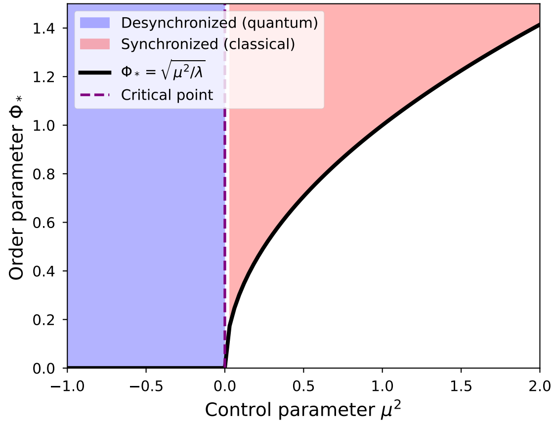
(b) Phase diagram
