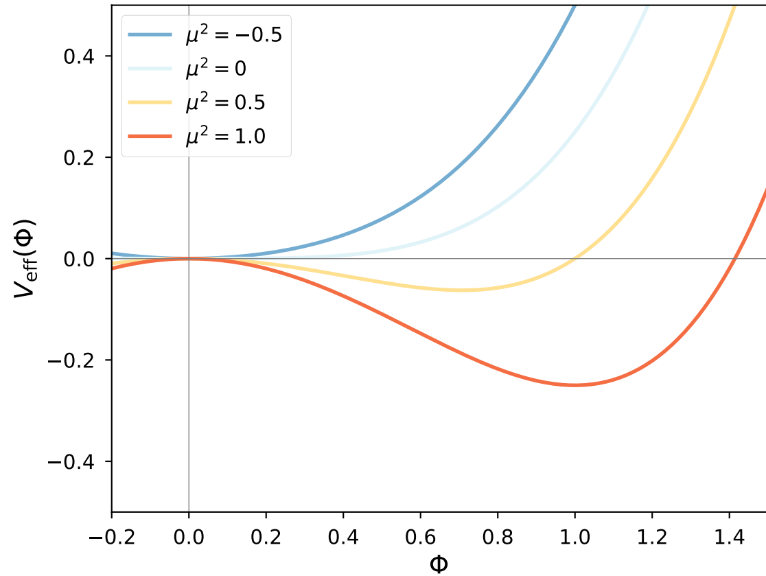
(a) Effective potential
