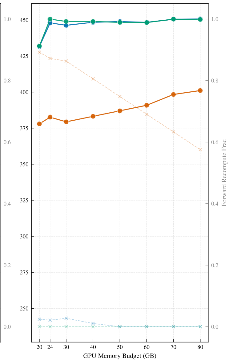
Sparse 16Bx3B, SeqLen 64K
