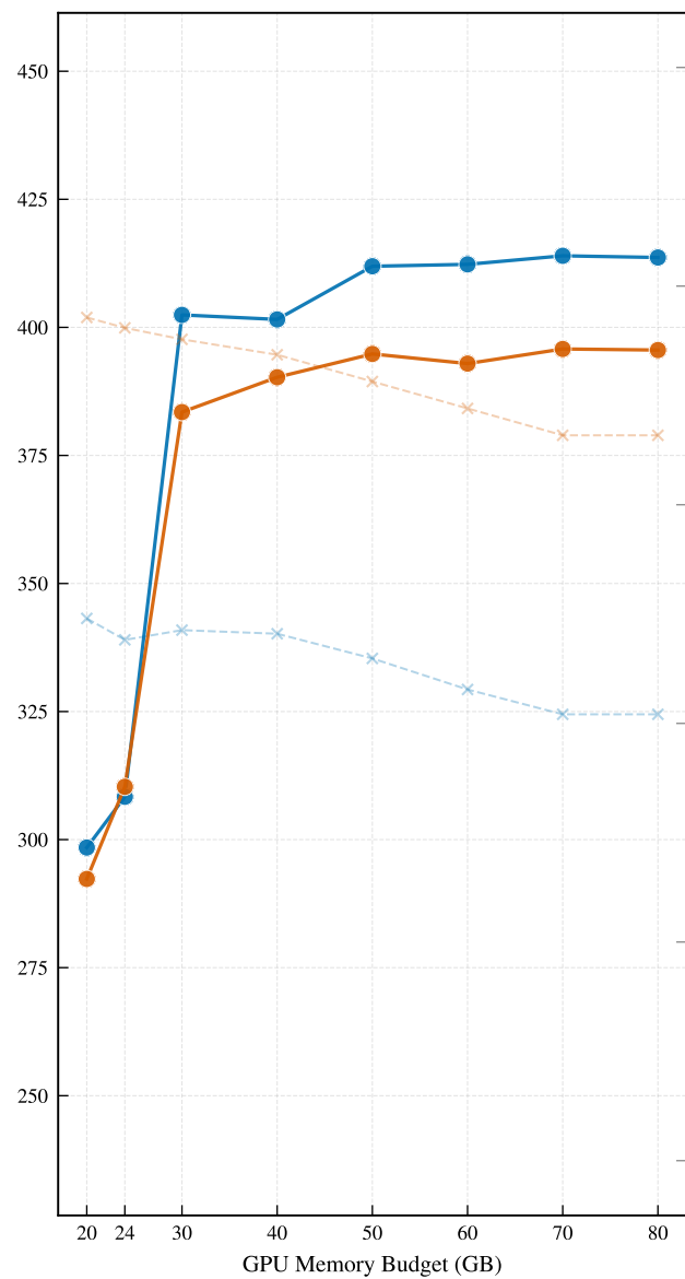
Sparse 16Bx3B, SeqLen 8K
