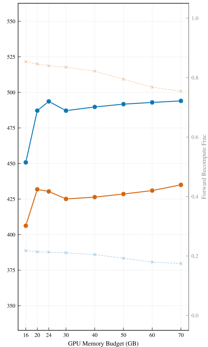
Dense 15B, SeqLen 64K
