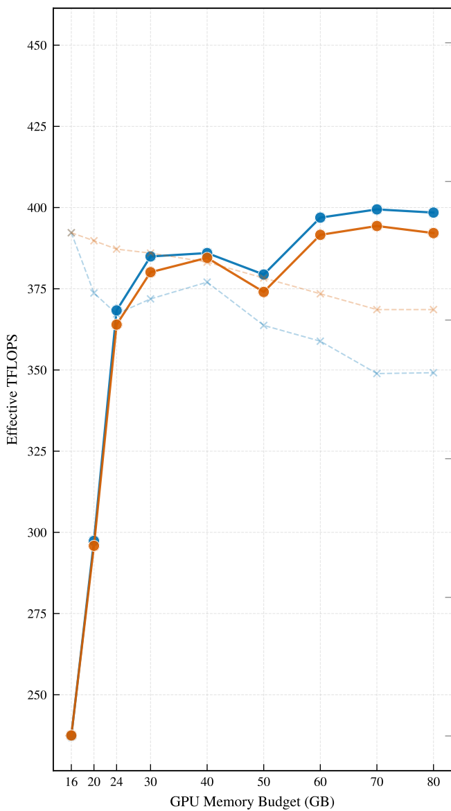
Sparse 16Bx3B, SeqLen 1K
