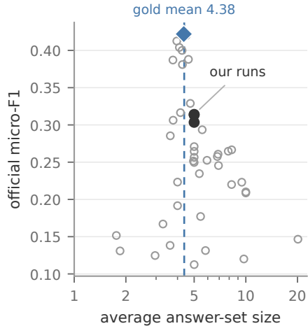
(a) Task 1
