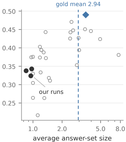
(b) Task 2
