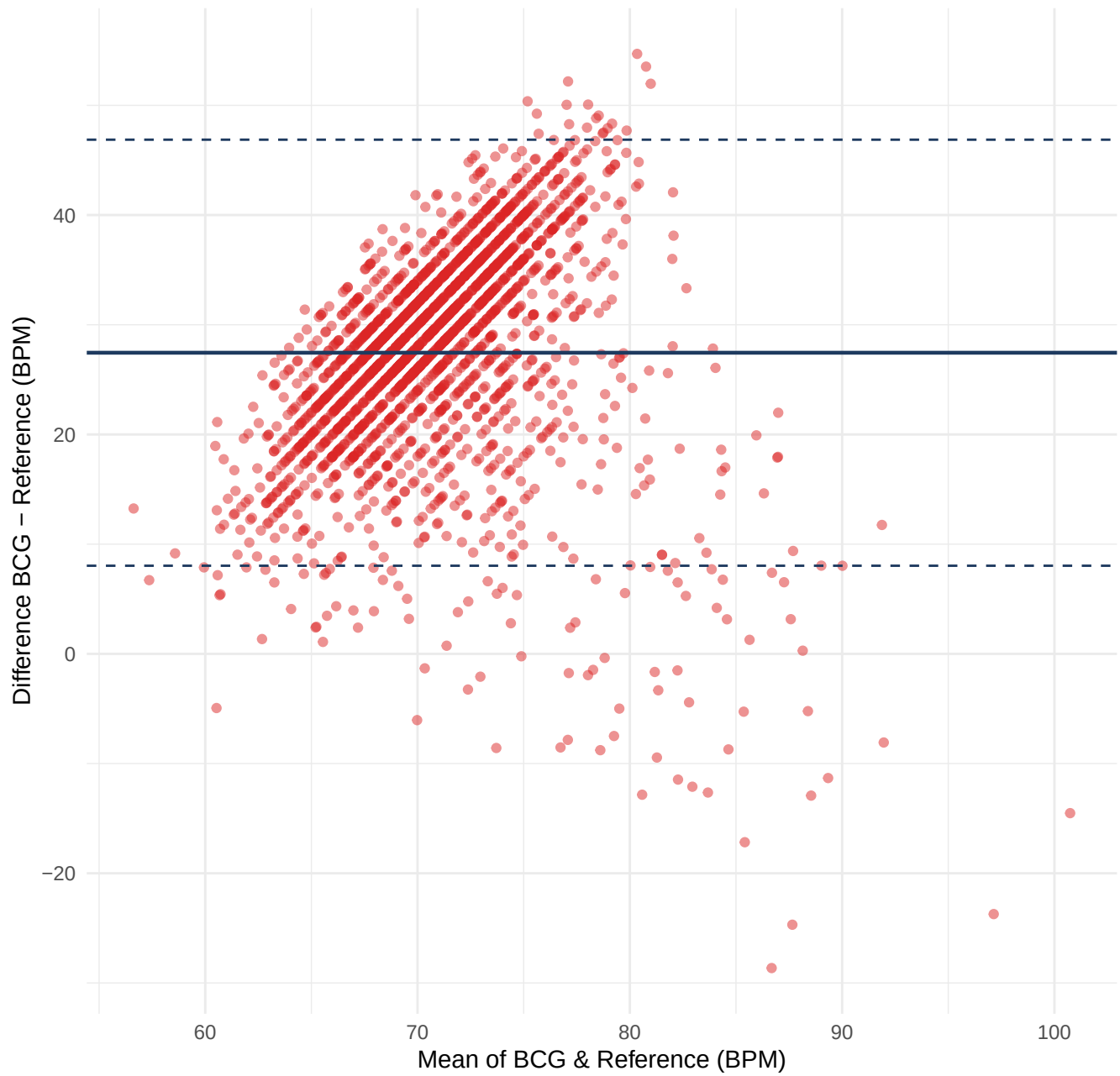
Bland-Altman
