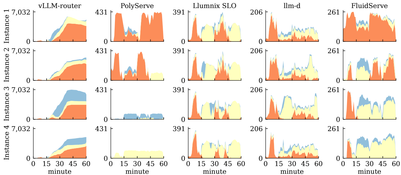
Requests resident per instance (own scale per column)
