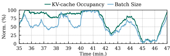
(a) Observed Engine State of an Instance
