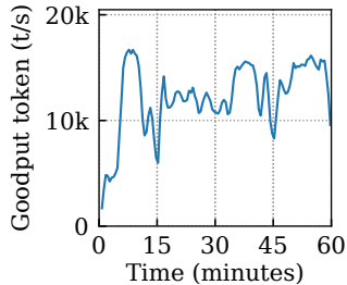
(b) Token goodput
