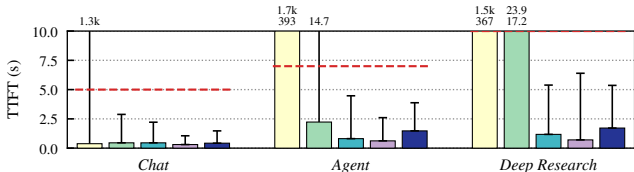
(a) Time to First Token (bar P50, whisker P95)
