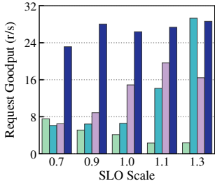
(b) Request Goodput
