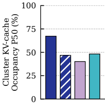
(a) KV-cache
