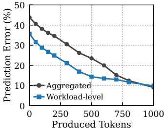
(a) Prediction Error
