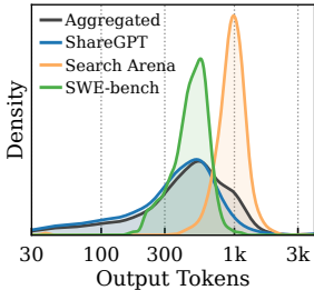
(b) Length Distribution
