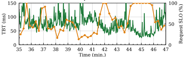
(c) Measured TBT and Request SLO Attainment of an Instance
