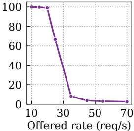
SLO attainment (%)
