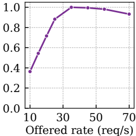
Normalized throughput
