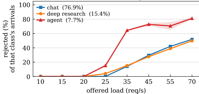
FluidServe refuses the agent class
