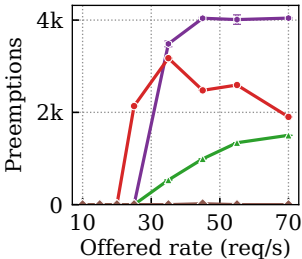
(a) Preemptions
