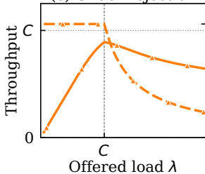
(c) Under-rejection
