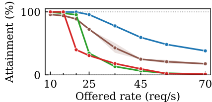
(c) Request SLO attainment
