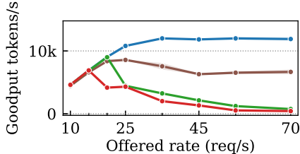
(b) Goodput tokens
