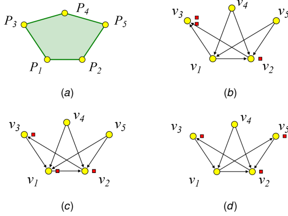
Fig. 4 (a) and (b): A P -cluster and its block representation. (c) and (d): Two consecutive pebble redistributions—first from v_3 to v_1 , then from v_1 to v_5 .
