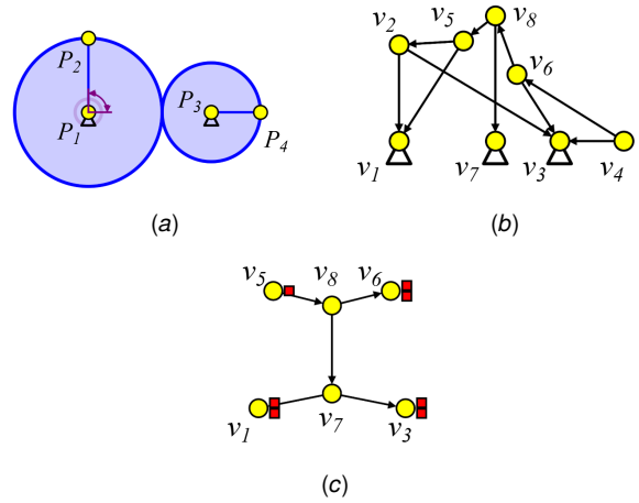
Fig. 11 11(a), 11(b), and 11(c): Simple gear train system, its constraint graph, and its conceptual edges
