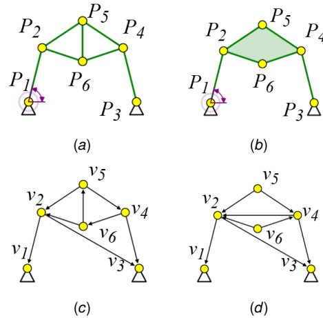
Fig. 6 6(a): Initial Structure; 6(b): Reduced Structure; 6(c): Possible Pinned Graph 1; 6(d): Possible Pinned Graph 2
