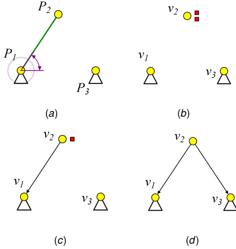
Fig. 2 Pebble assignment in a simple planar mechanism during pinned constraint graph construction
