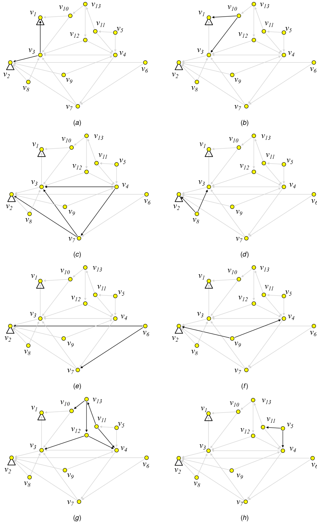
Fig. 13 Solving steps for the planar geared linkage system in 12(a). The edges colored in black correspond to the constraint equations for the respective solving steps.
