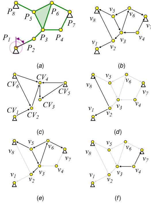
Fig. 5 5(a) and 5(b): P -vertex-only linkage mechanism and its graph representation; 5(c): Condensed graph; 5(d), 5(e), and 5(f): Consecutive Assur graphs in the mechanism
