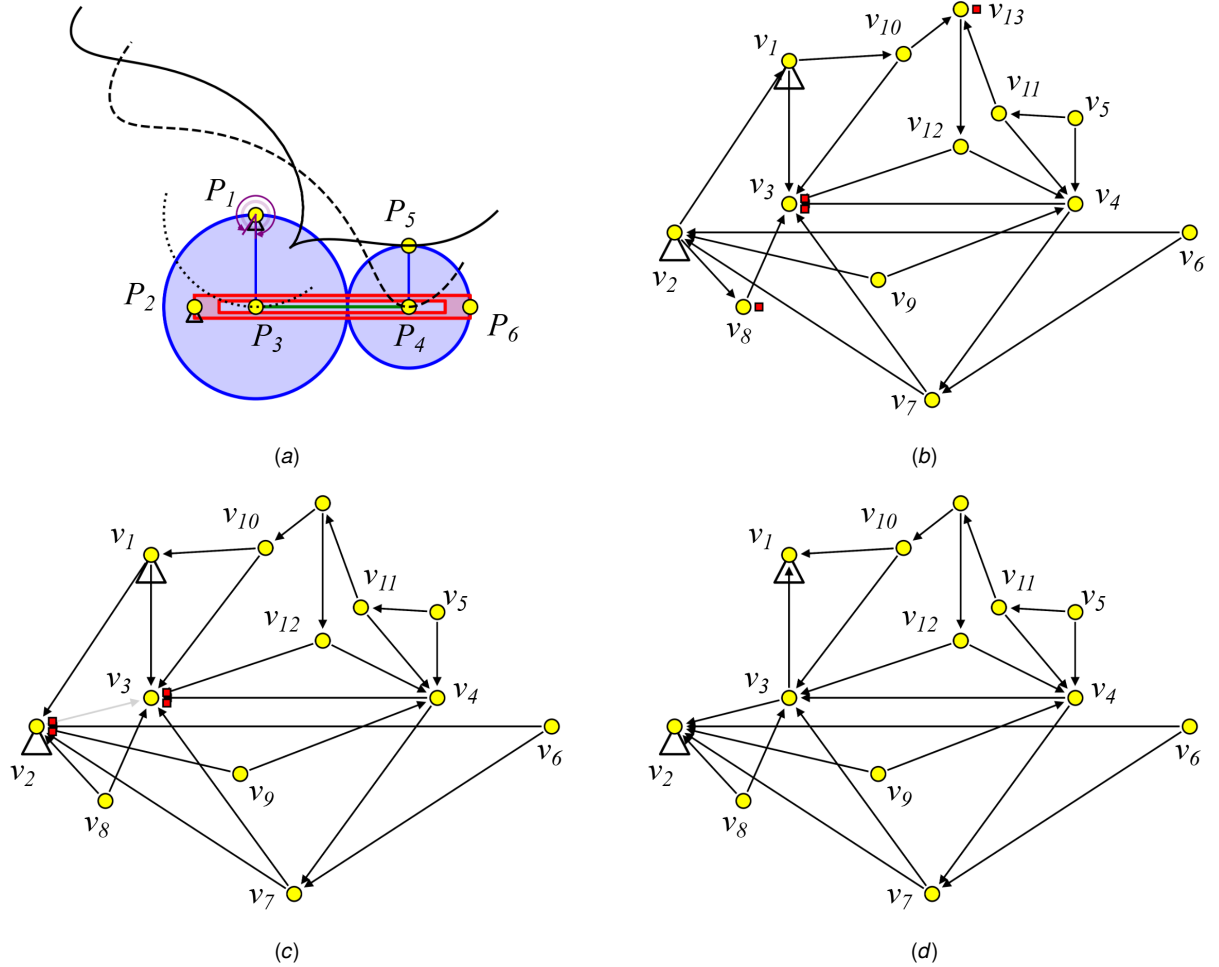
Fig. 12 12(a): Planar geared linkage; 12(b): Reduction result; 12(b): Constraint graph before the dynamic edge insertion; Figure 12(c): Constraint graph after the dynamic edge insertion; Figure 12(d): Constraint graph after pinning the ground vertices
