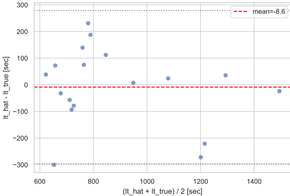
Bland-Altman Lin25_899597df (lt2, policy=median)
