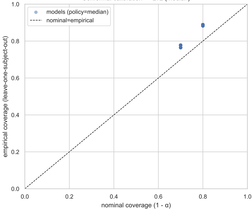
Conformal calibration — LT2 (median)
