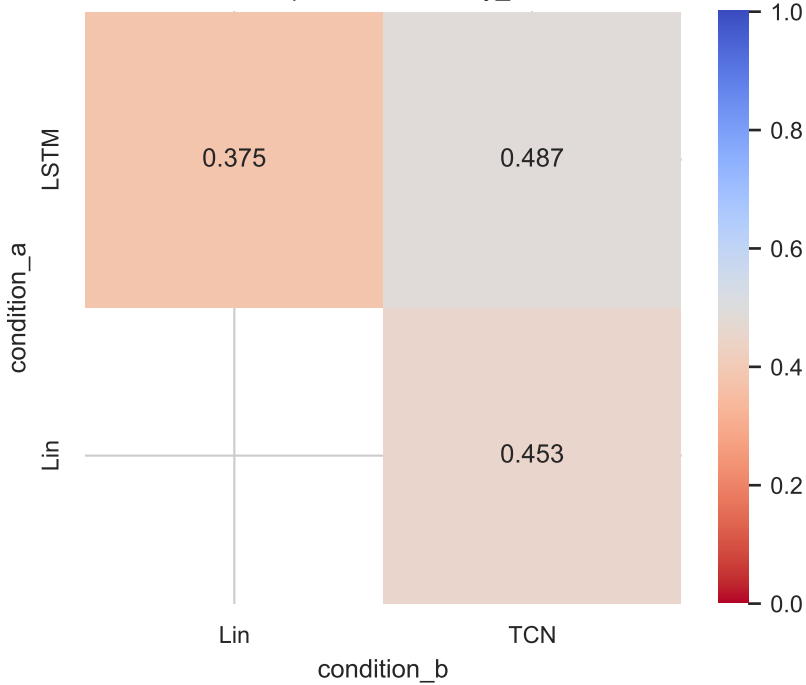
Wilcoxon p-values — family_overall
