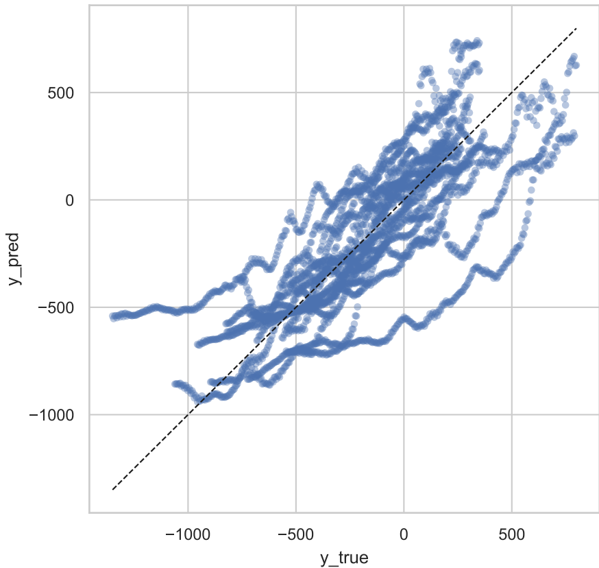
Pred vs GT — LSTM3_31f2b090
