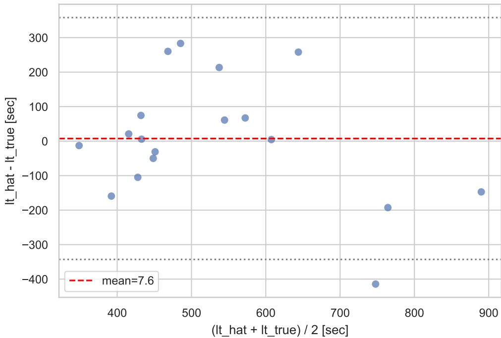
Bland-Altman Lin25_9d4fb194 (lt1, policy=median)
