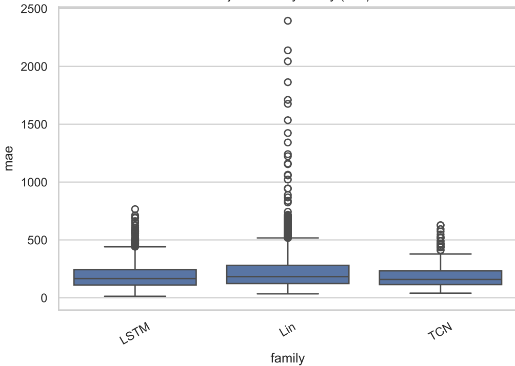
Subject MAE by family (LT2)
