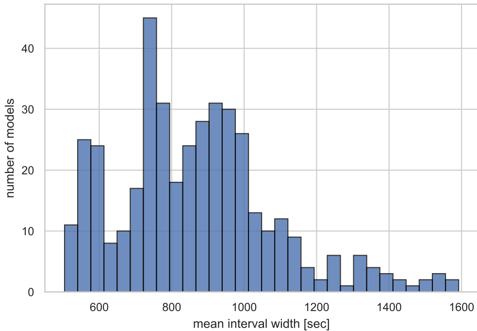
Conformal width — LT1 (median, \alpha=0.2 )
