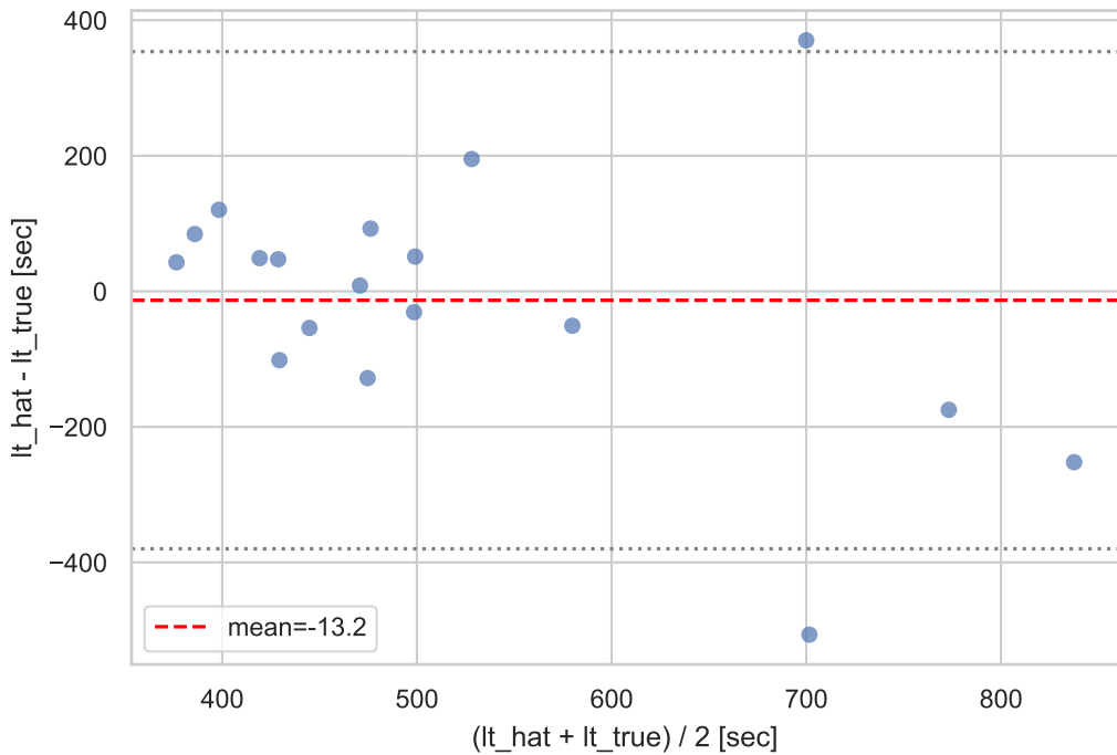
Bland-Altman LSTM3_31f2b090 (lt1, policy=median)
