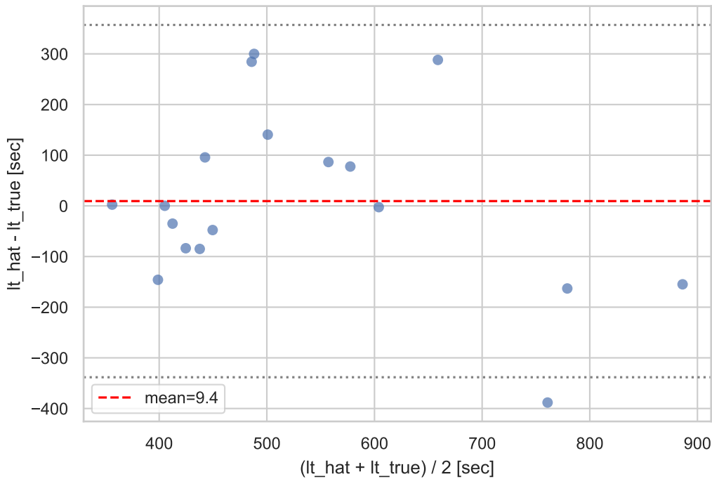
Bland-Altman Lin24_e86acbf9 (lt1, policy=median)
