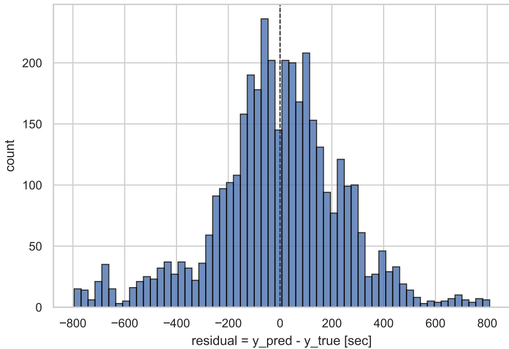
Error histogram — LSTM3_31f2b090
