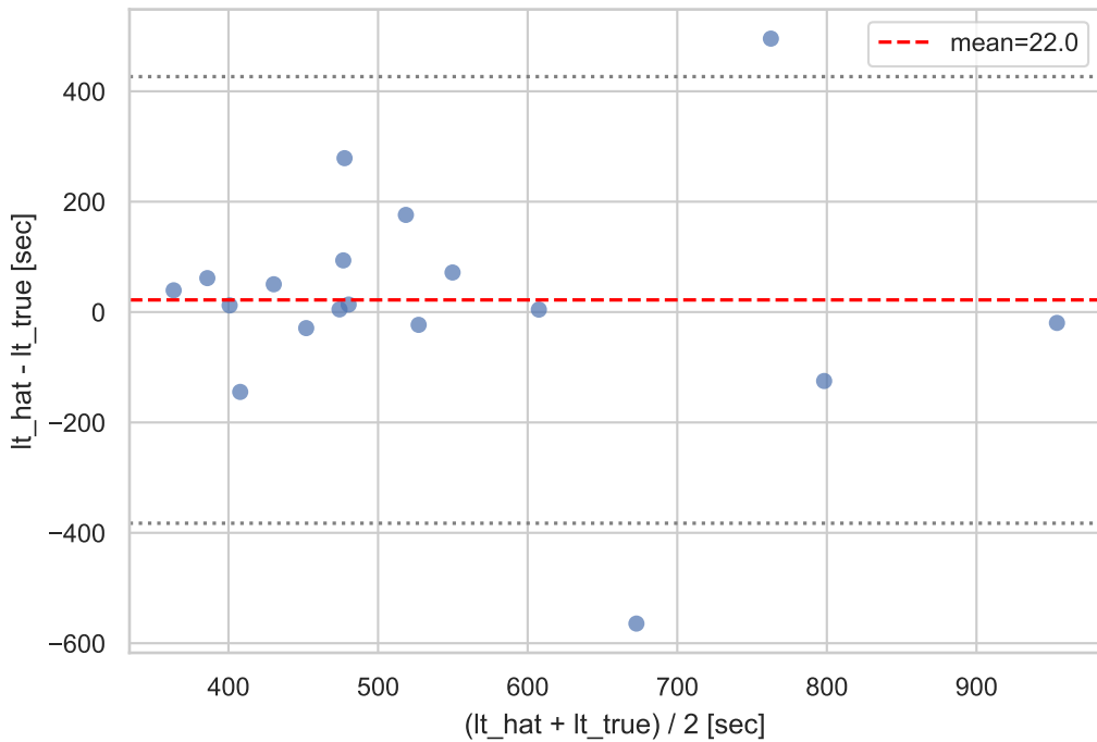
Bland-Altman Lin14_228f08a1 (lt1, policy=median)
