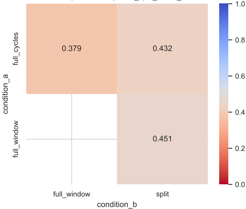
Wilcoxon p-values — phase_split_within_arch
