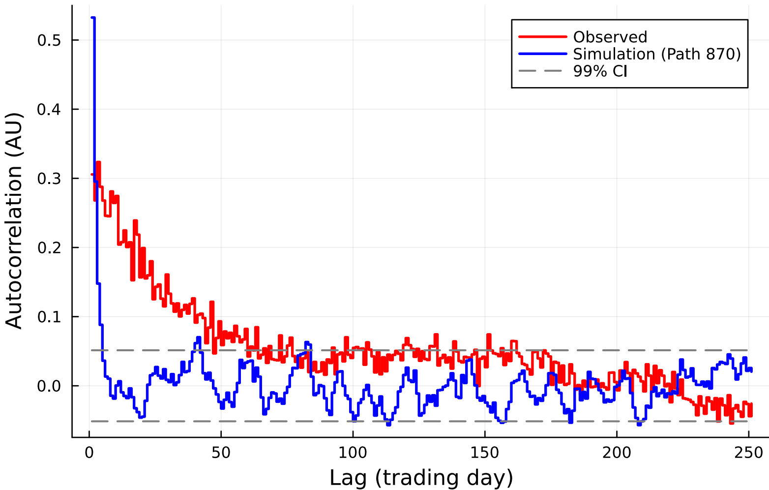
ACF of SPY |Growth Rate| (Jump, Path 870)
