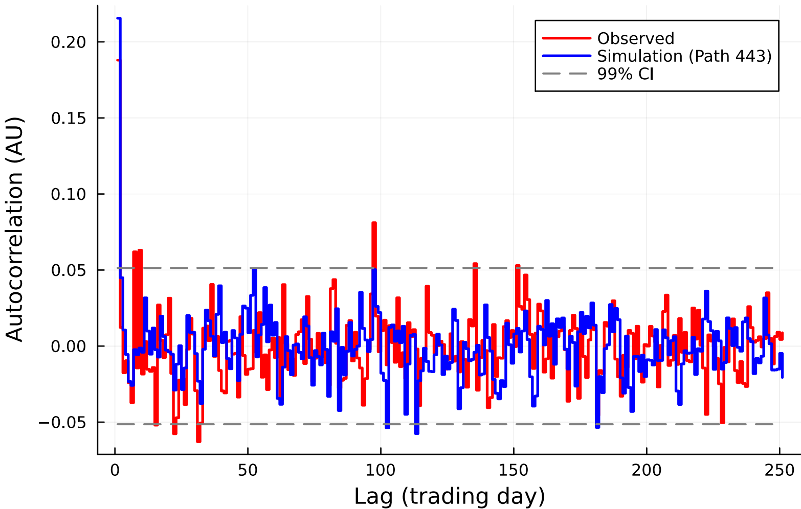
ACF of SPY Growth Rate (Jump, Path 443)
