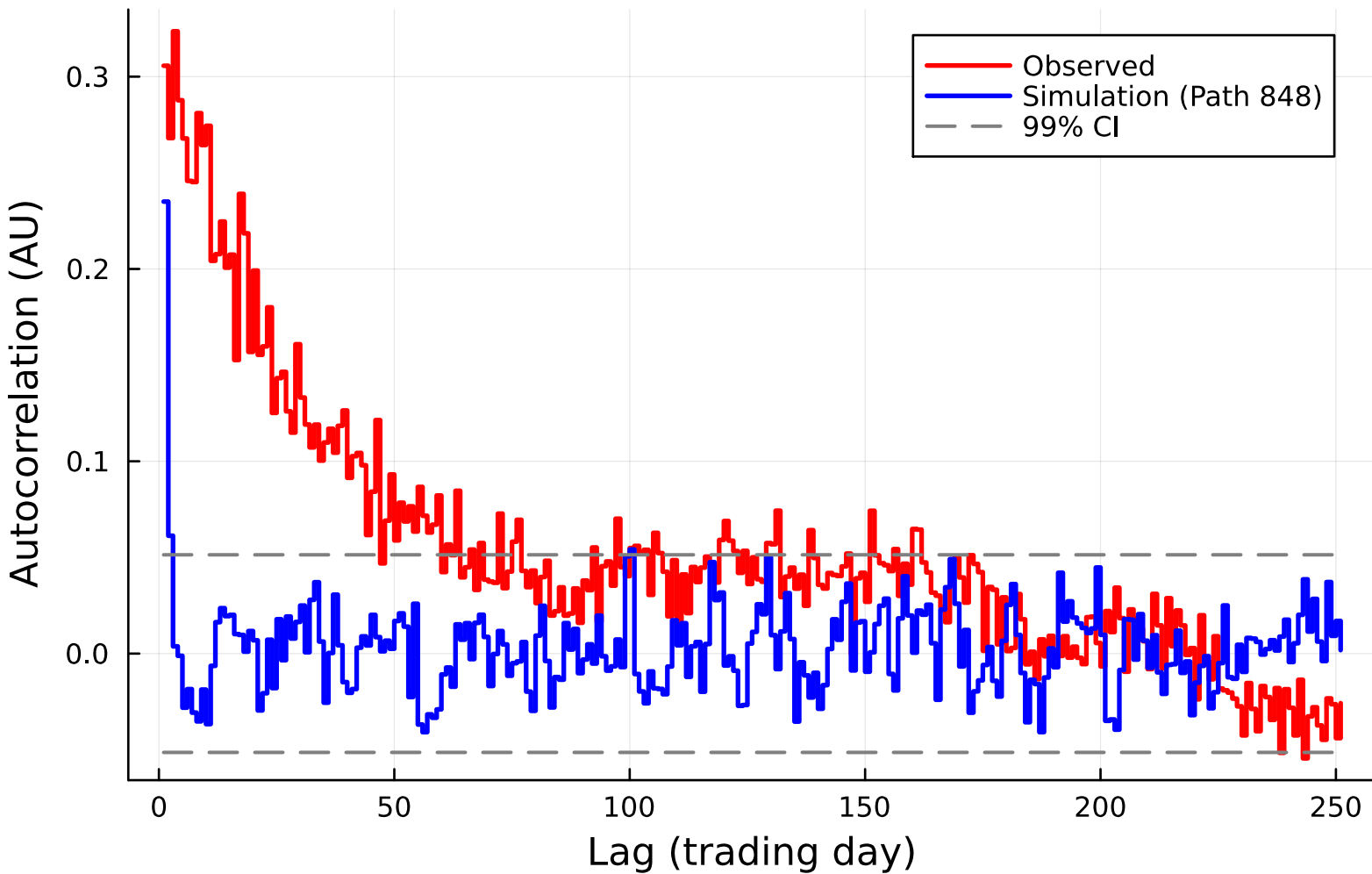
ACF of SPY |Growth Rate| (Jump, Path 848)
