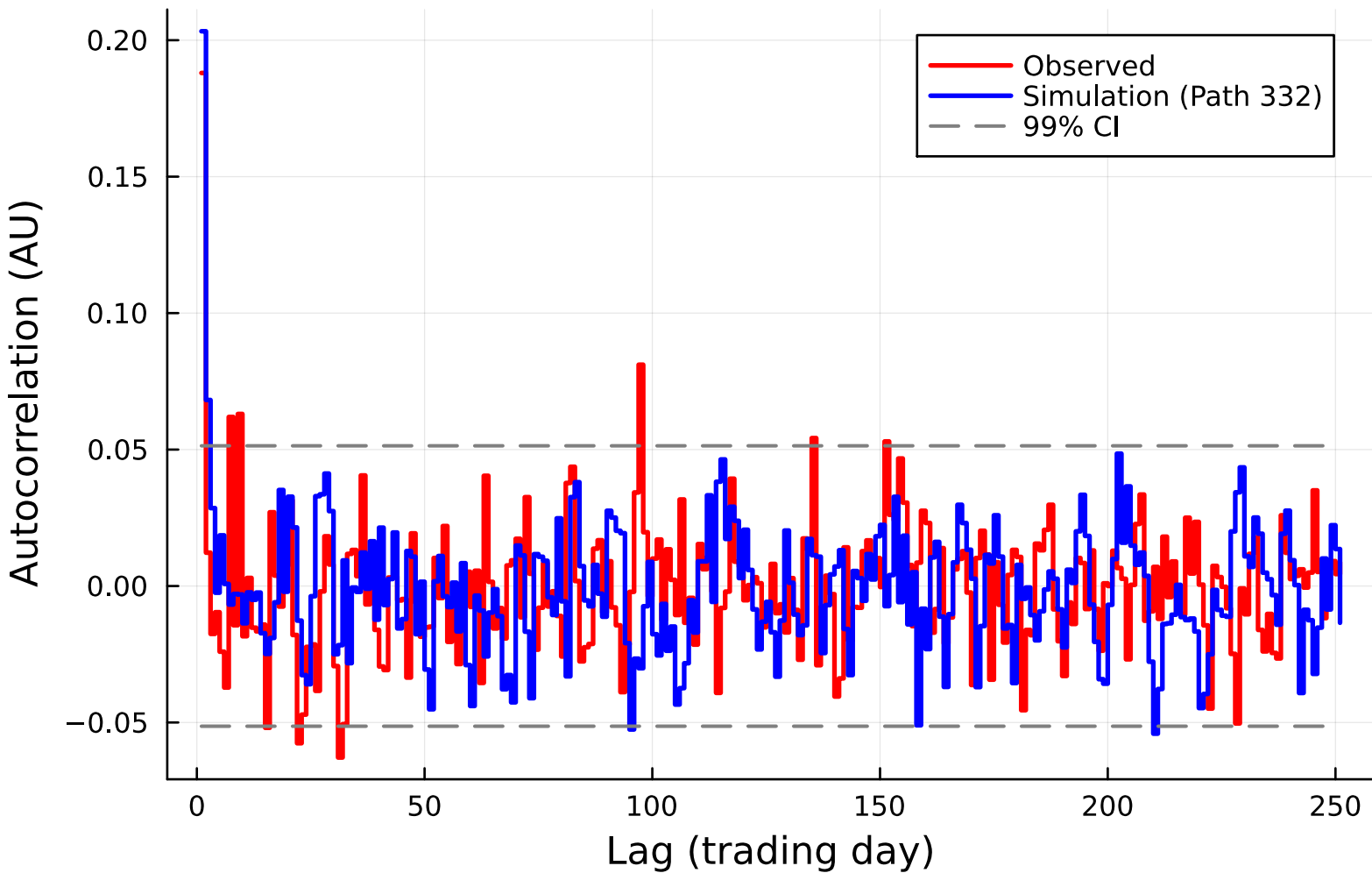
ACF of SPY Growth Rate (Jump, Path 332)
