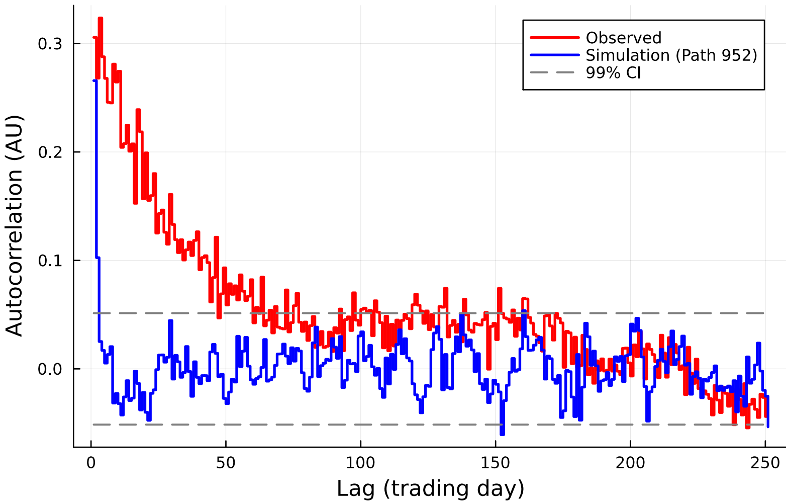
ACF of SPY |Growth Rate| (Jump, Path 952)
