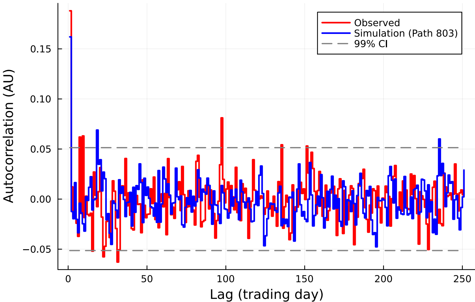
ACF of SPY Growth Rate (Jump, Path 803)
