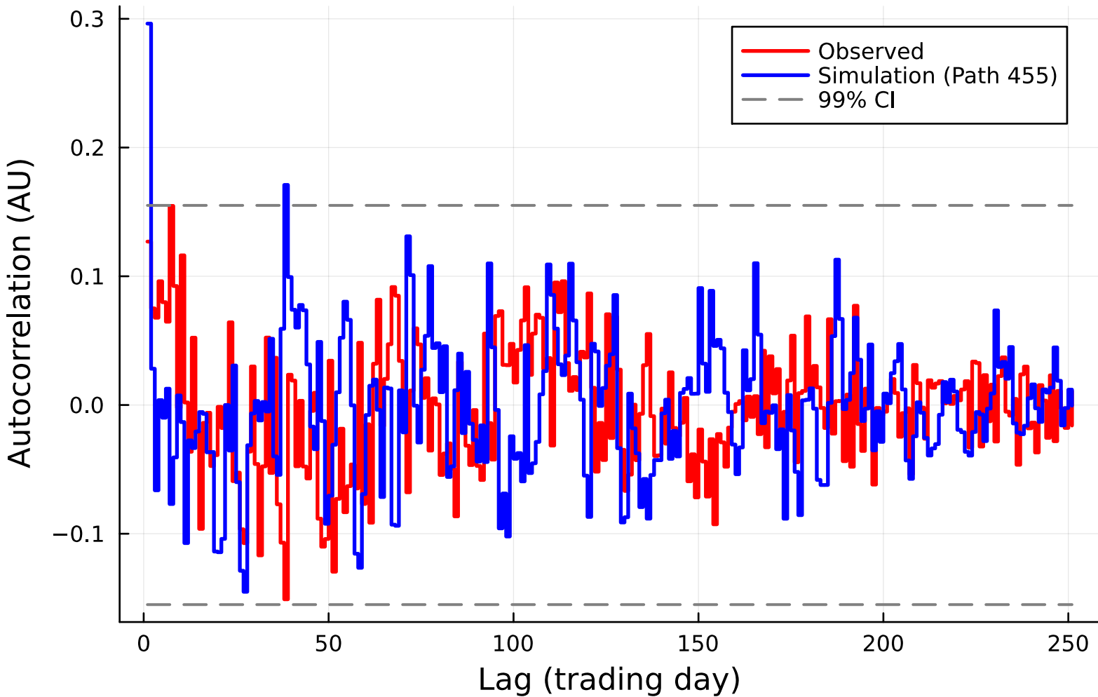
ACF of SPY [Growth Rate] (Jump, Path 455)
