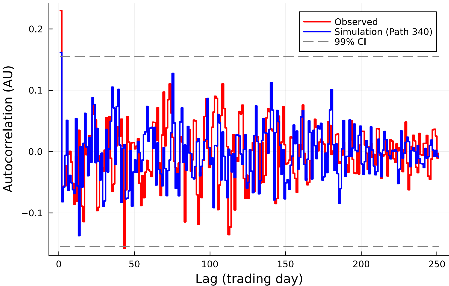
ACF of SPY Growth Rate (Jump, Path 340)
