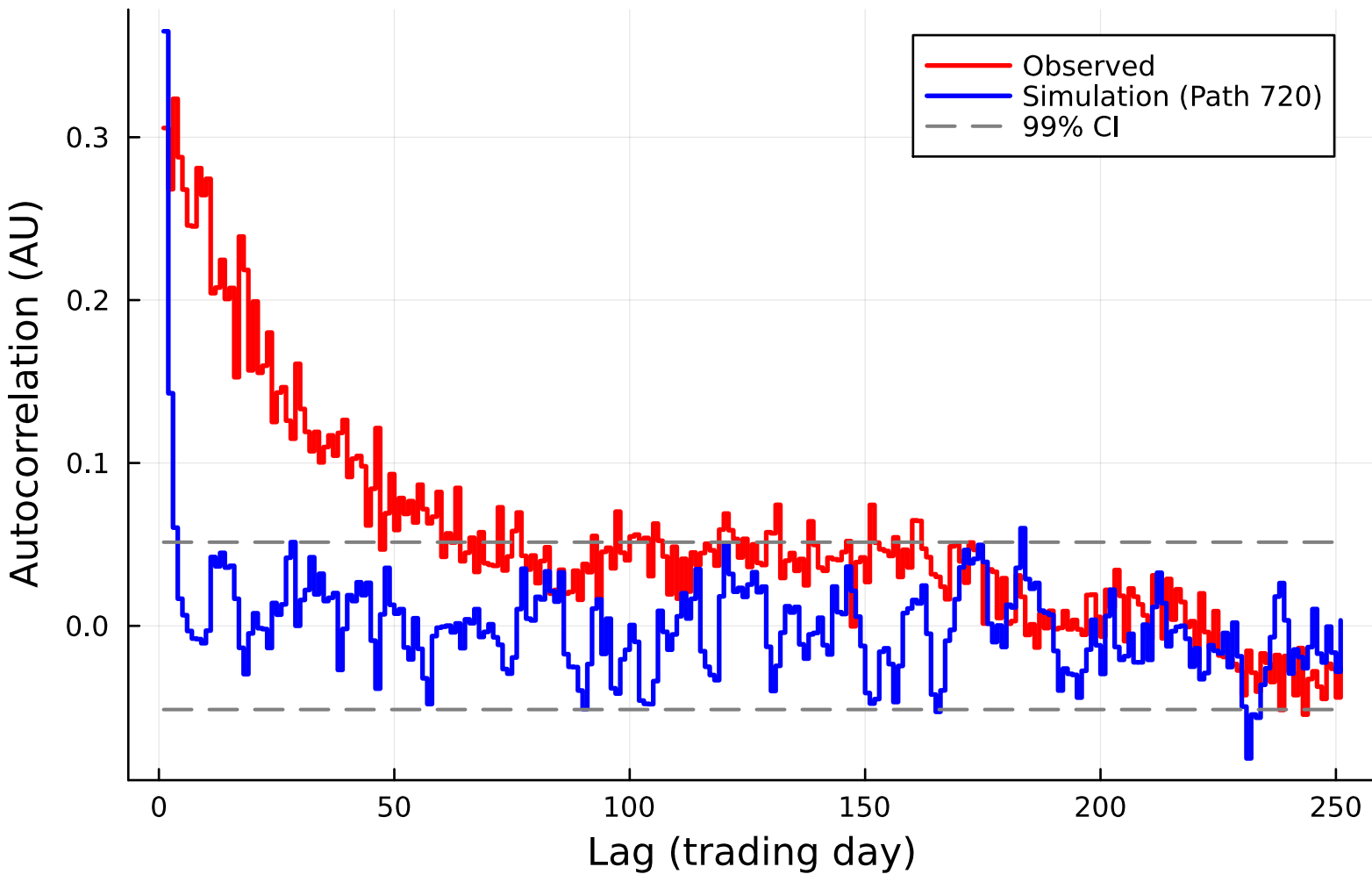
ACF of SPY |Growth Rate| (Jump, Path 720)
