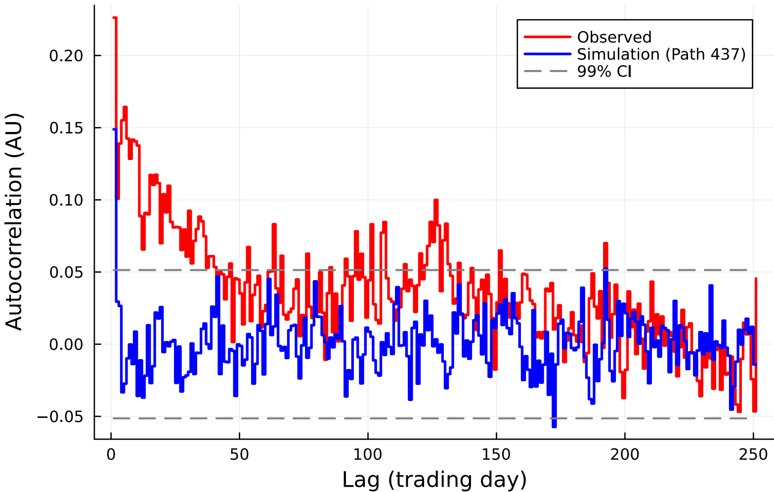
ACF of AAPL |Growth Rate| (Jump, Path 437)
