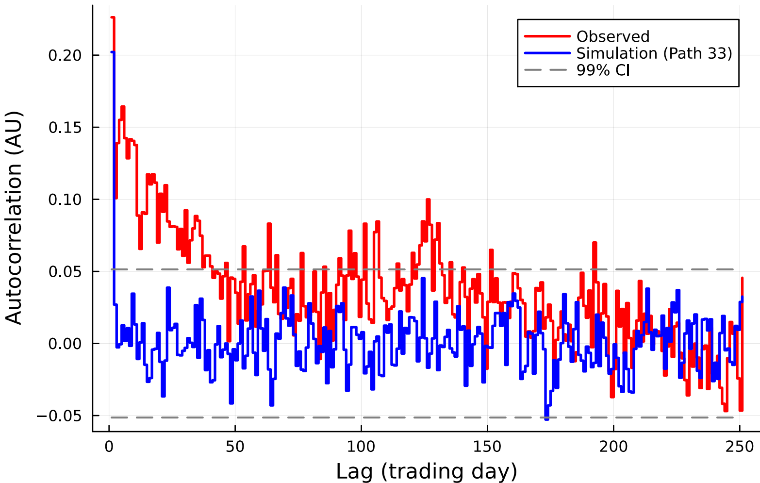
ACF of AAPL |Growth Rate| (Jump, Path 33)
