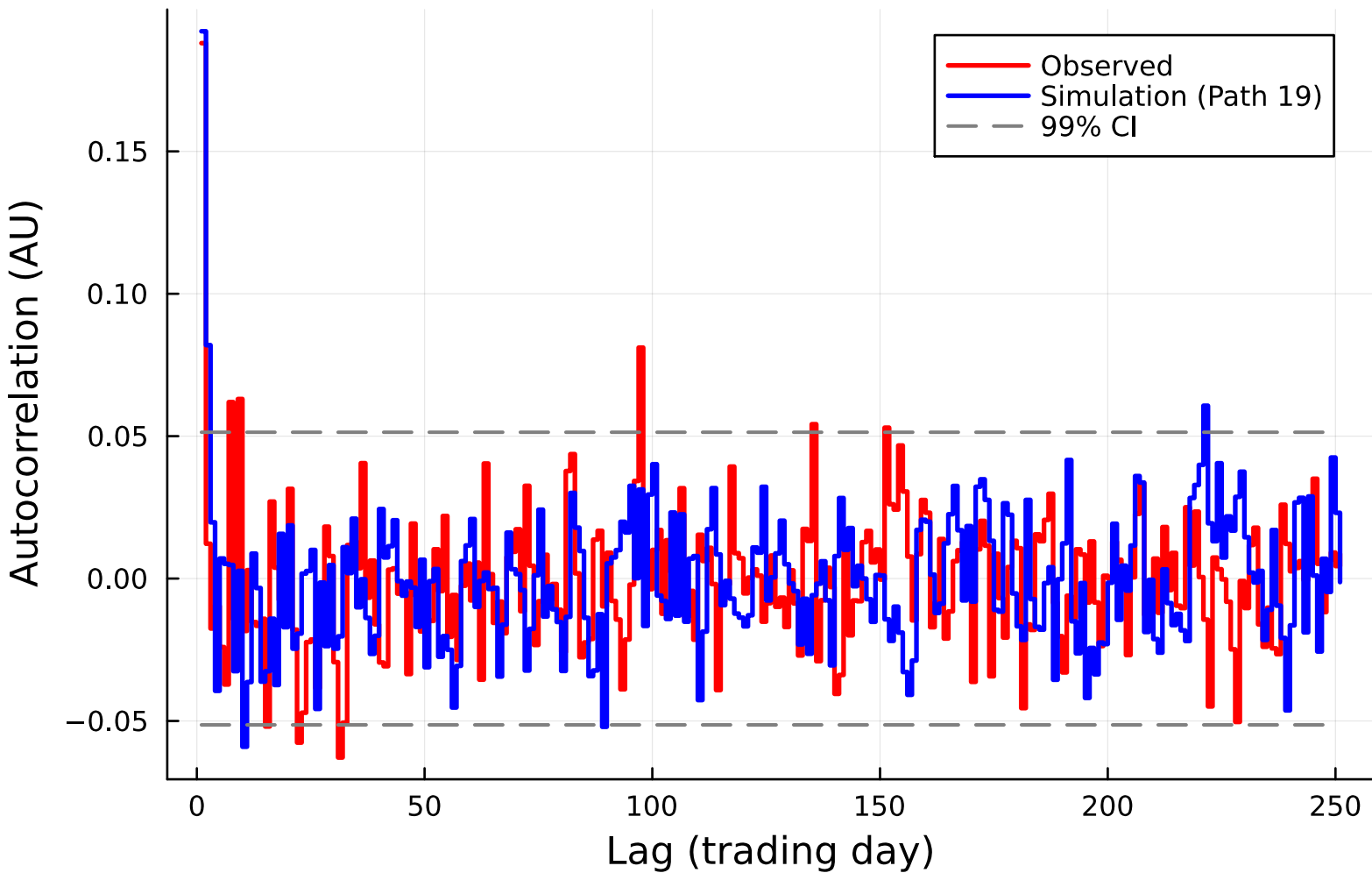
ACF of SPY Growth Rate (Jump, Path 19)
