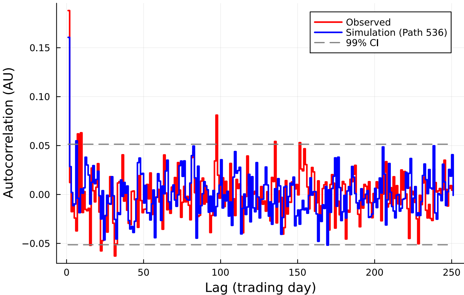
ACF of SPY Growth Rate (Non-Jump, Path 536)
